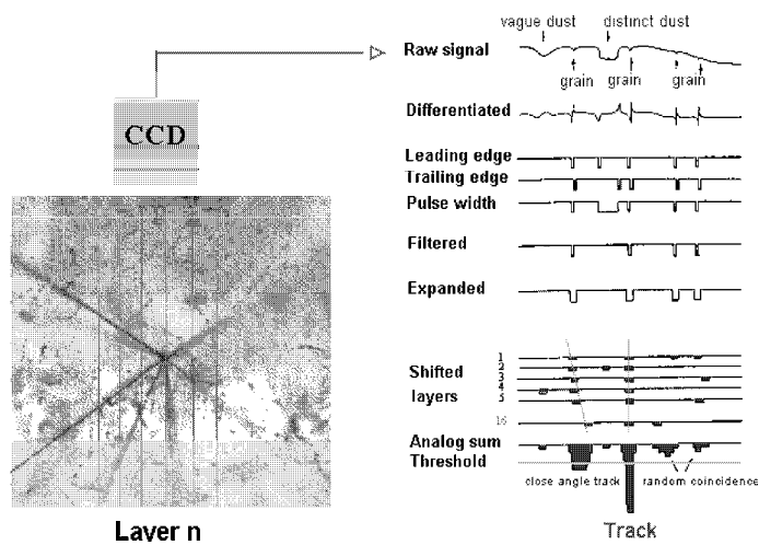
Figure VI.3: Schematic representation of the image processing done by the Track Selector to find the signal associated to predicted tracks.
