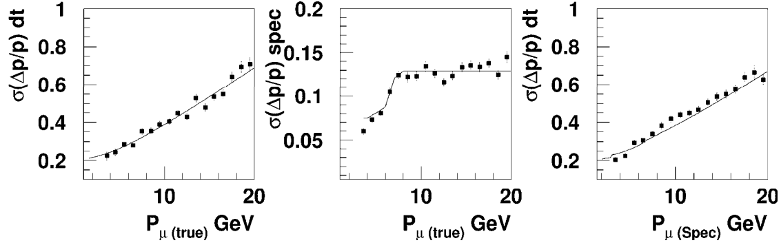
Figure V.13: Momentum resolution for muons coming from simulated \nu_\mu interactions. Each dot represents the sigma of the distributions of \frac{P_{\text{measured}} - P_{\text{reference}}}{P_{\text{measured}}} in bins of P_{\text{reference}} . Left : The momentum measured in the air-core magnet is compared to the true (simulated) momentum. Centre : The muon spectrometer momentum corrected for the energy loss in the calorimeter is compared to the true momentum. Right: The momentum measured in the air-core magnet is compared to the muon spectrometer momentum corrected for the energy loss in the calorimeter. The lines show the result of a fit to the data (left and centre plots), and the quadratic combination of the 2 fits (the right plot).
