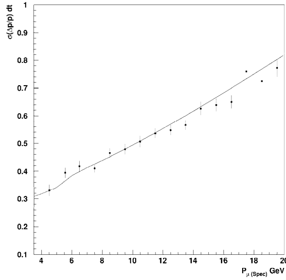
Figure V.15: Momentum resolution for muons from neutrino CC interactions : the momentum measured in the air-core magnet is compared to the muon spectrometer momentum corrected for the energy loss in the calorimeter. Each dot represents the sigma of the distributions of \frac{P_{fibre}-P_{spec}}{P_{fibre}} in bins of P_{spec} . The curve shows the combined resolution of the two spectrometers, the errors are statistical.
