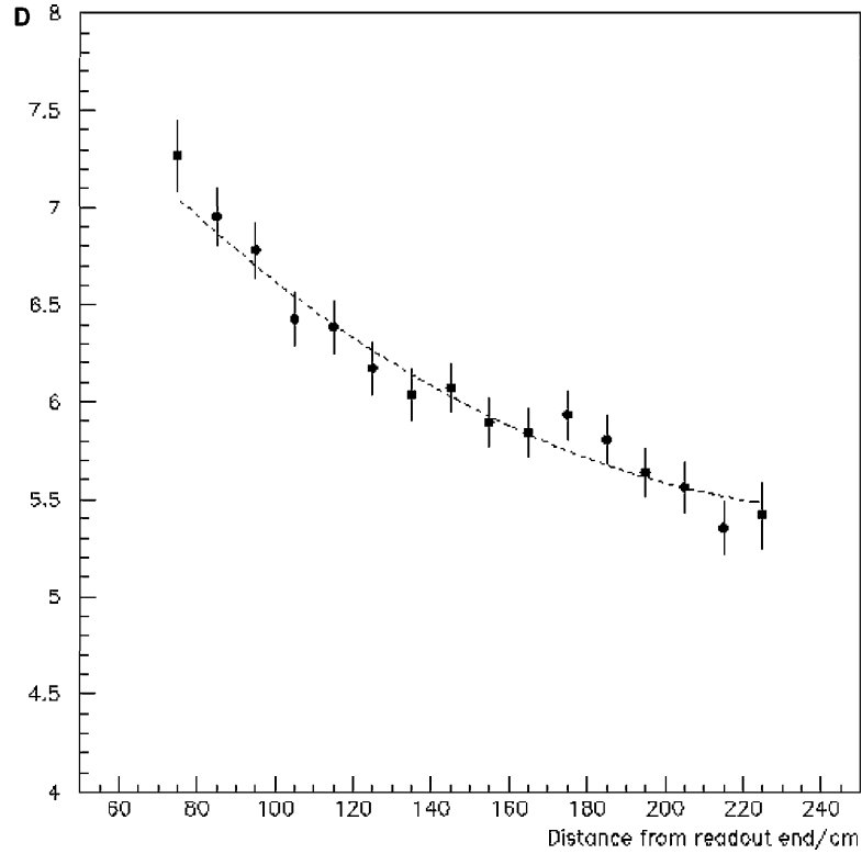
Figure IV.5: Density of hits from a minimum ionising particle as a function of the distance from the readout end
