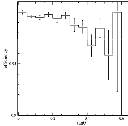
Figure VI.4: Track Selector Track finding efficiency as a function of the track slope with respect to the beam direction.
