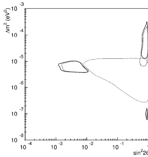
Figure II.3: Results of the four solar neutrino experiments, in terms of possible neutrino oscillations solutions. The shaded area is the region excluded at 99% C.L. by Super-Kamiokande non observation of day-night effects. The regions in the dotted lines are allowed at 99% C.L. by the rate comparison between BP98 and the Ga, Cl, and Super-Kamiokande, the solid lines is the region allowed at 99% C.L. by the rate comparison analysis and the day-night effect analysis.
