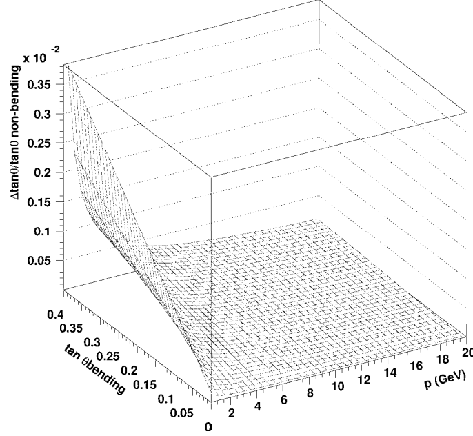
Figure V.8: Relative variation of the slope in the non-bending plane as a function of the slope in the bending plane and of the momentum
