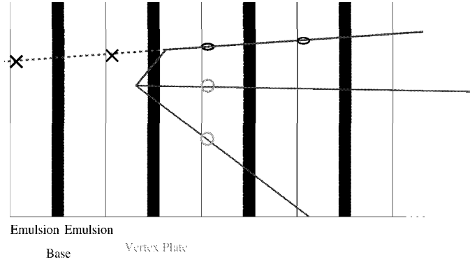
Figure VI.6: Illustration of the search for a \tau^- decay in the same plate as the primary \nu_\tau interaction vertex.
