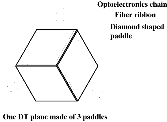
Figure IV.7: Front view of three paddles forming one DT plane. Each paddle contains 16 7-layers fibre ribbons and is readout by a separate optoelectronic chain.
