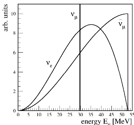
Figure II.7: Neutrino energy spectra from \pi^+ \rightarrow \mu^+ \nu_\mu decay at rest followed by \mu^+ \rightarrow \bar{\nu}_\mu e^+ \nu_e decay at rest.
