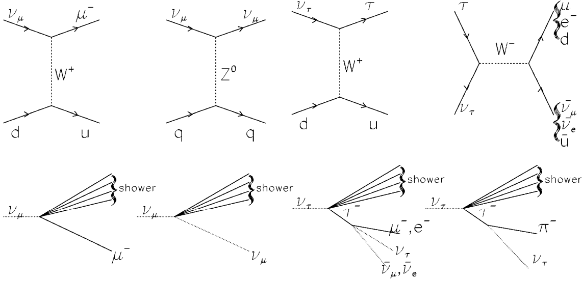
Figure III.2: Diagrams and topologies of the \nu_\tau CC interaction with the subsequent decay of the \tau^- .
